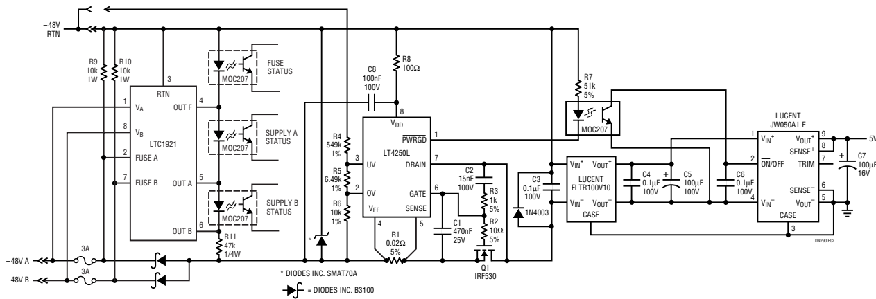
Figure 2. Network Switch Card Monitor with Hot Swap Control
